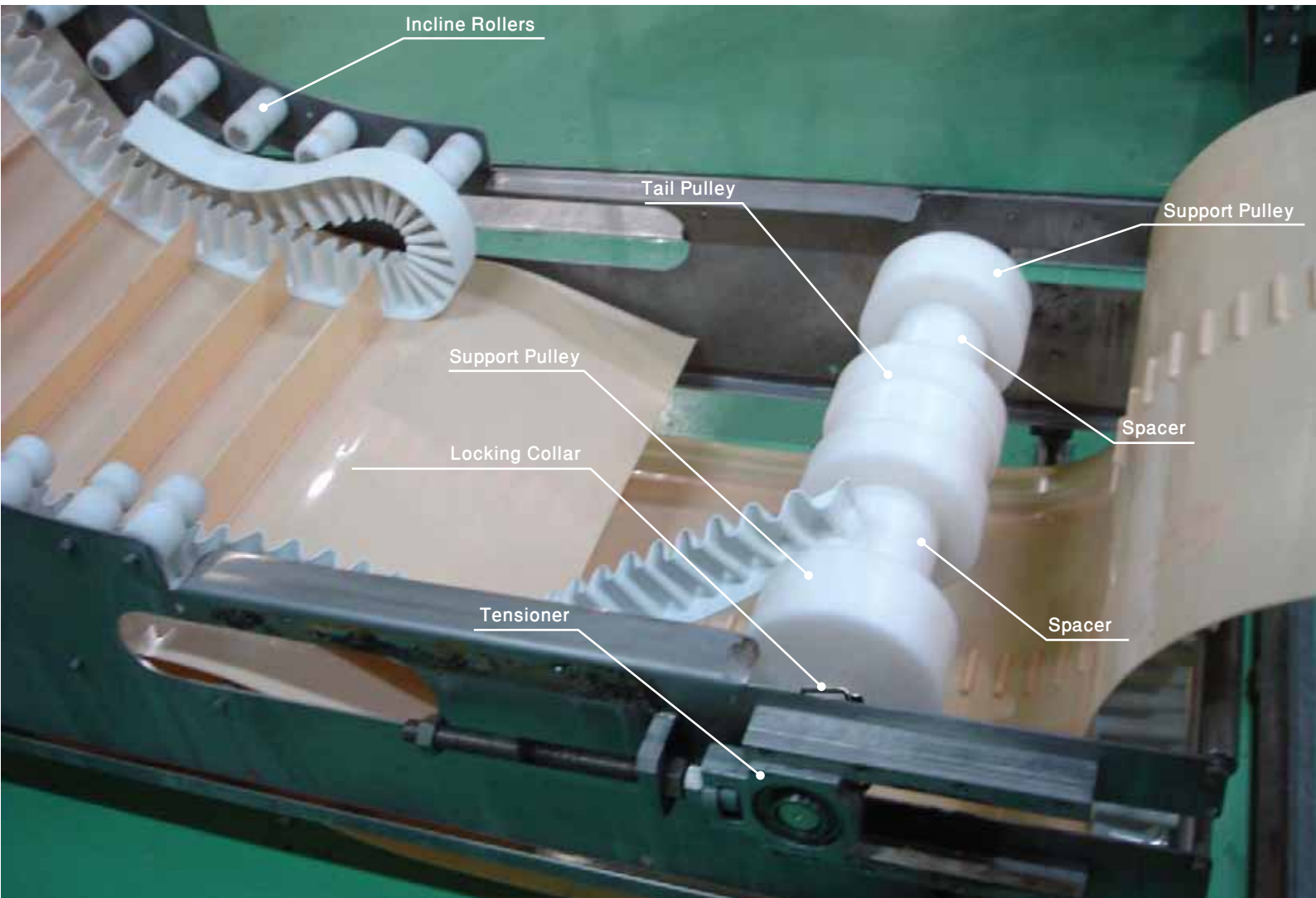
Fabricated SuperDrive™ Being Made Endless on Site
