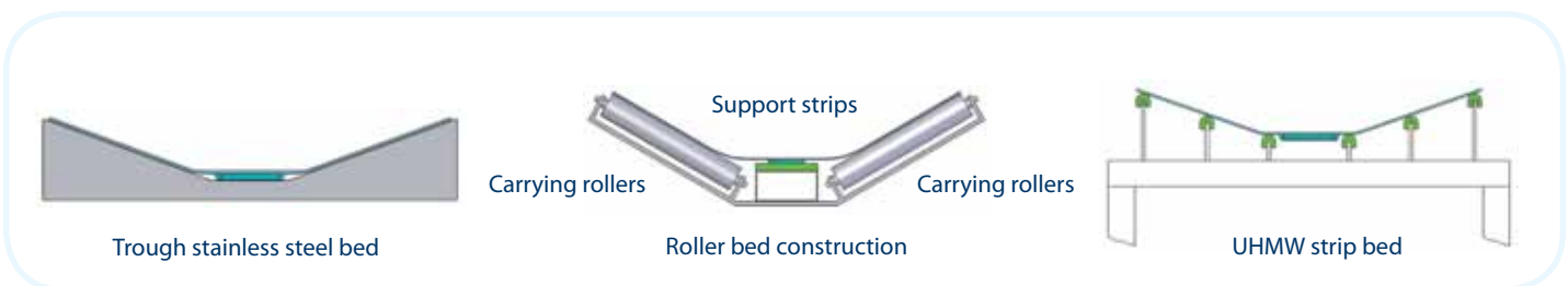
Trough Bed Construction Options
